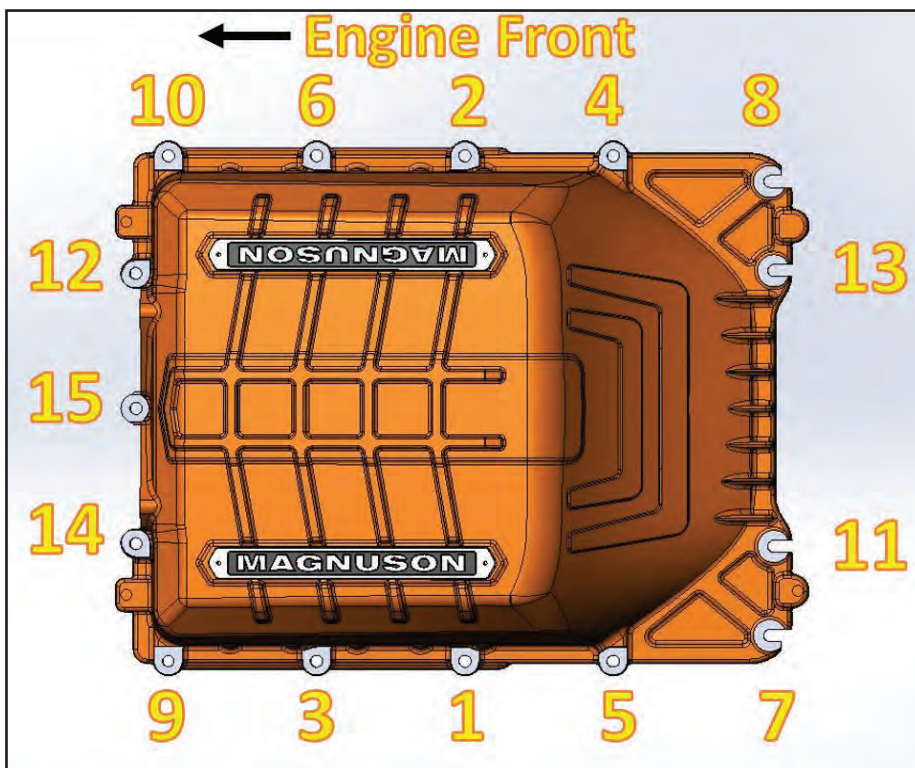
Lid Torque Sequence (18 ft-lbs. Final Torque)
